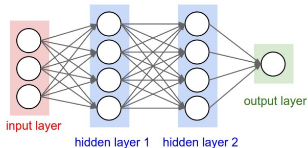
Feedforward network
