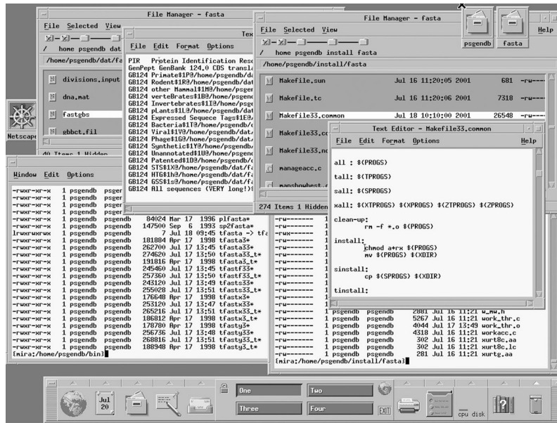
Fig. 2. Leveraging the multiwindow desktop. In the example, the environment variable $DB, which identifies the root directory for bioinformatics software, is set to /home/psgen db. Clockwise from top left: Double clicking on fastgbs in $DB/doc/fasta opens up a list of locations of database files in a text editor. Similarly, Makefile33.common has been opened up from $DB/install/fasta. This file contains Makefile commands that are compatible with all operating systems. A terminal window at lower right is used for running commands in $DB/install/fasta, while another terminal window at bottom left is used for running commands in $DB/bin. At bottom, the CDE control panel shows that the current screen, out of four screens available, is screen One.
