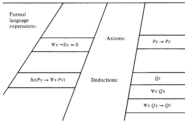
Figure 8. The meta-language above, in which we study the object language below.
