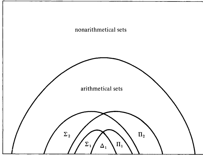
Figure 10. Picture of \mathcal{P}\mathbb{N} .
